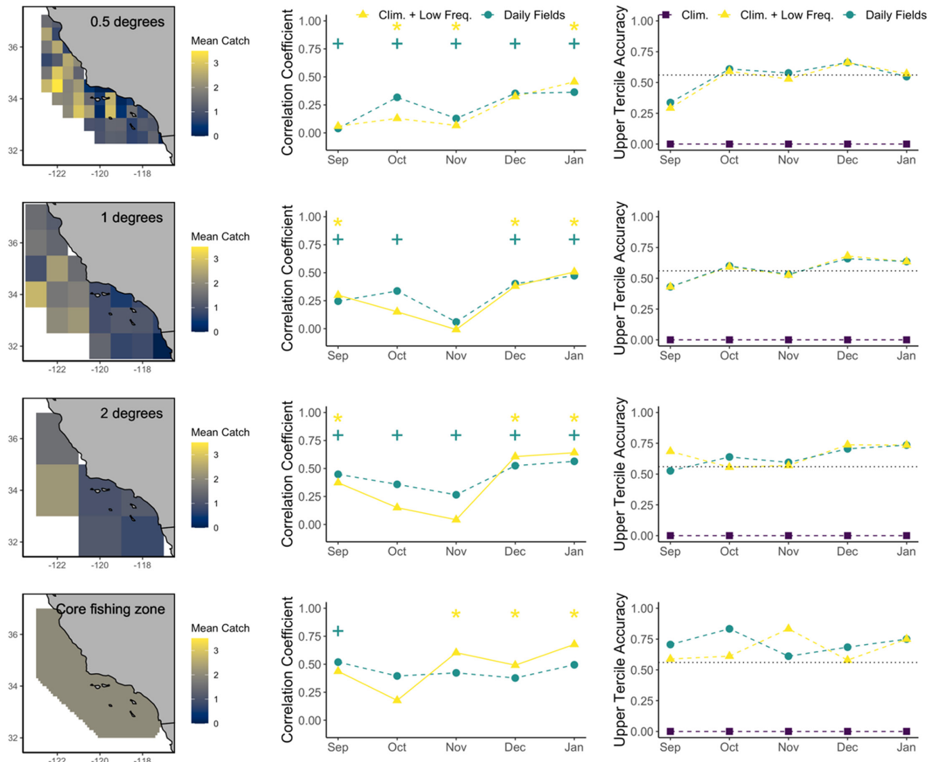
Figure 4. Average observed swordfish catch (maps) and predictive performance for modeled swordfish catch anomalies, with predictions averaged over four spatial resolutions ( 0.5^\circ , 1^\circ , 2^\circ and the entire region). Anomaly correlation coefficients (middle column) and probabilistic accuracy (right column) are shown for each month for the daily values species distribution model (blue circles), the monthly climatology plus low frequency model (yellow triangles), and the monthly climatological model (purple squares). Blue crosses and yellow stars indicate significance of the correlation coefficients ( p < 0.05 ). The horizontal black line at 0.56 indicates the minimum level of probabilistic accuracy, with values below this no better than random. Correlation coefficients for the monthly climatology are 0 and not shown.
